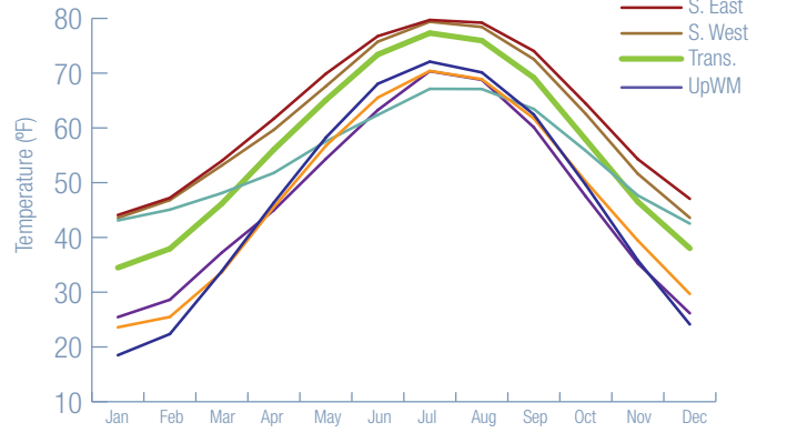
Figure 80. 30-yr monthly average temperature in the Transition region.
