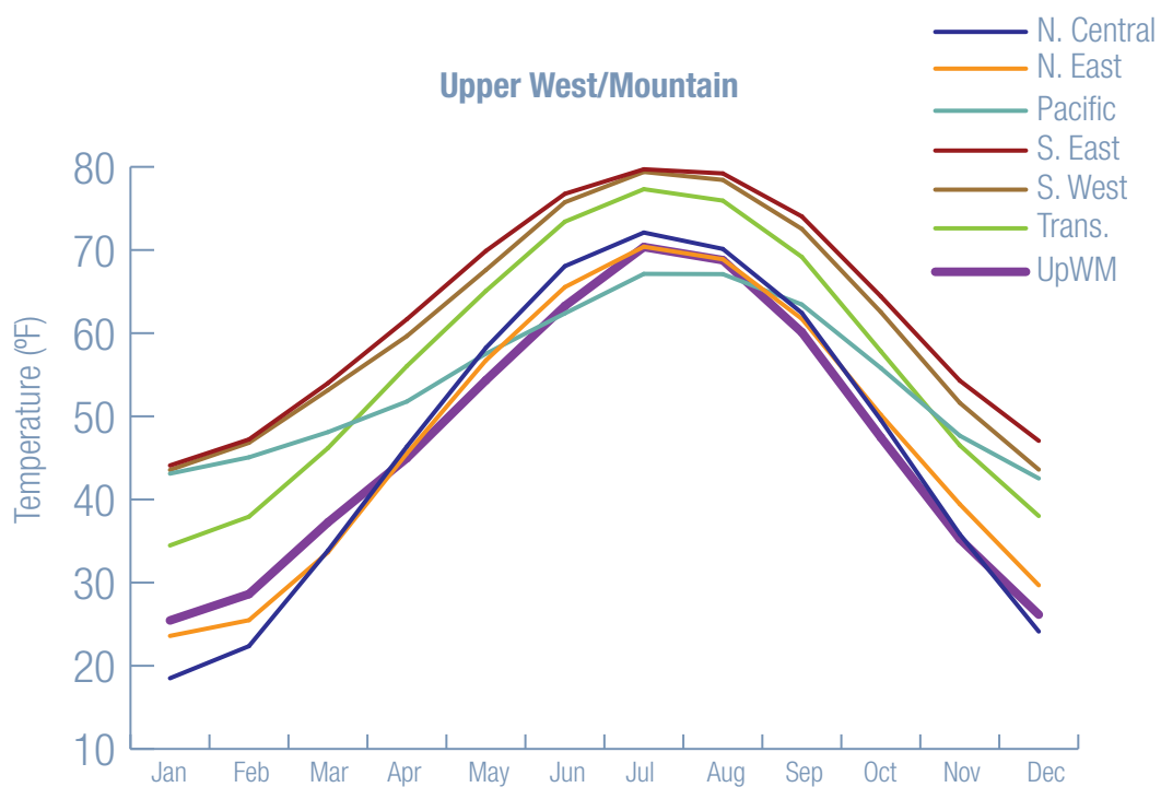
Figure 92. 30-yr monthly average temperature in the Upper West/Mountain region.
