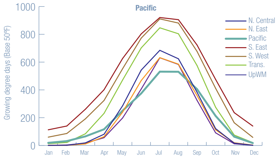
Figure 45. 30-yr monthly average growing degree days in the Pacific region.
